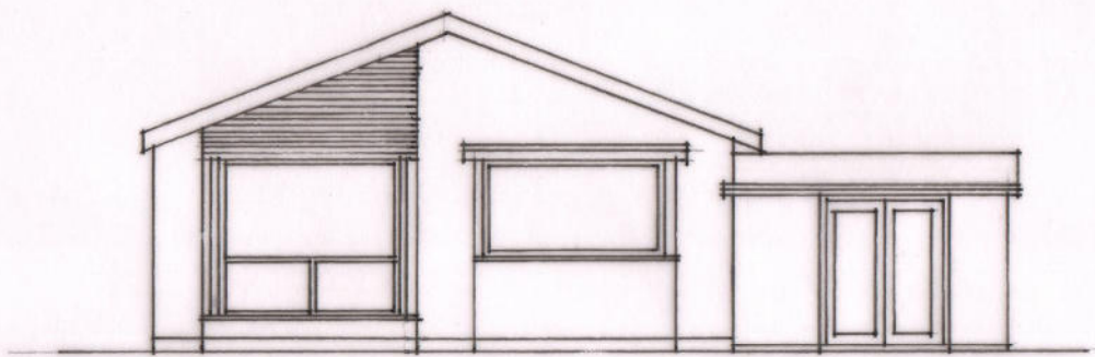
EXISTING REAR ELEVATION 1:100
